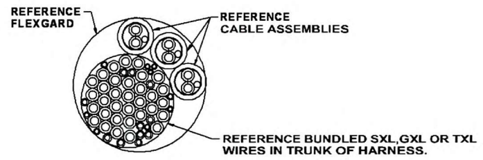
DETAIL BDR WIRE/CABLE BUNDLING
